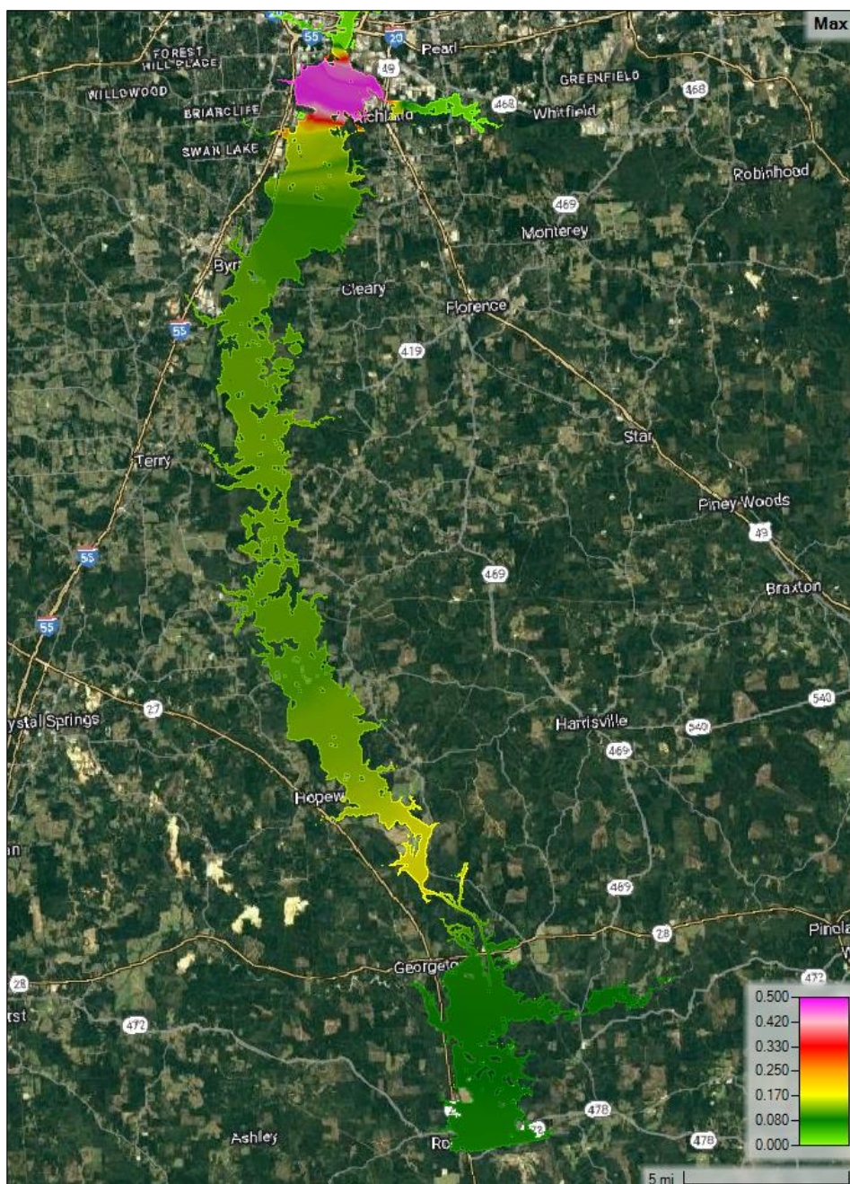
Figure E5-15. 5-year Frequency Absolute Differences (Feet) for With and Without Project. Figure shows the additional height due to Alternative C or CTO construction added to the maximum water surface elevation for the 5-year frequency event. (All areas in yellow or green are less than the 0.25 feet, which is considered unlikely to have substantive inducements after further analysis.)
